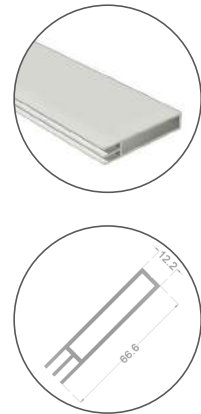
Aluminiumprofil 67 mm:
