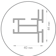
Aluminiumprofil 44 mm offen:
